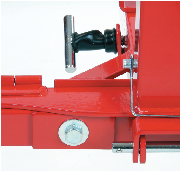
When assembling P/N 410-020 Outer Cross Support Tube, be sure to use the enclosed rectangular washers along with the round flat washers (4X).
