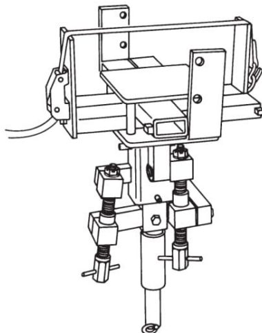
No. 540233 Universal Transmission Adapter Assembly (optional)
