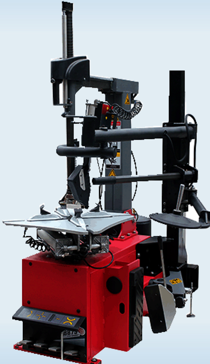
TC-1300 Leverless Tire Changer
