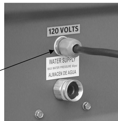
Electrical cord for 120V, 20Amp connection. Note: Standard 3/4" water connection for utility water source under 60 p.s.i.
